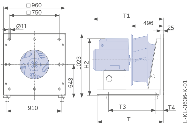
Dimensions mm
