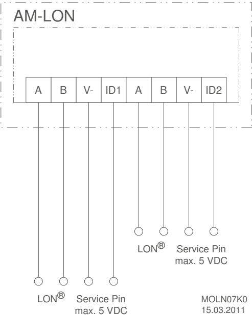
Connection diagram
