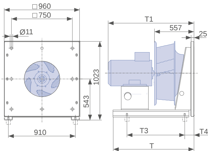
Dimensions mm
