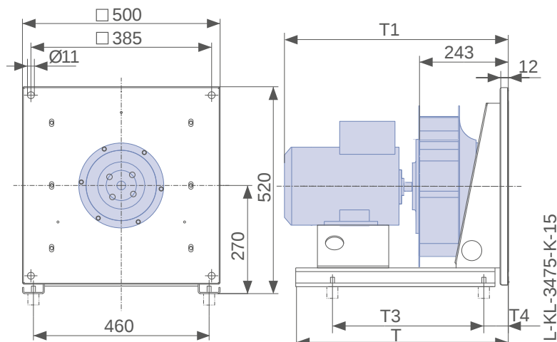
Dimensions mm
