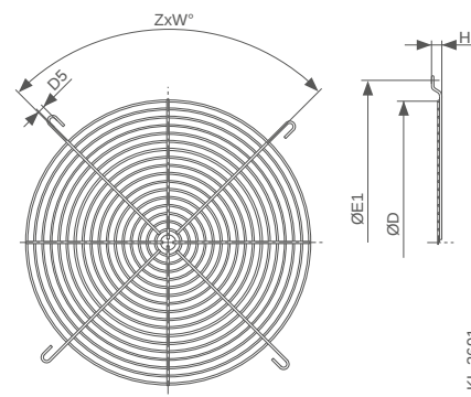
Guard grille on suction side
