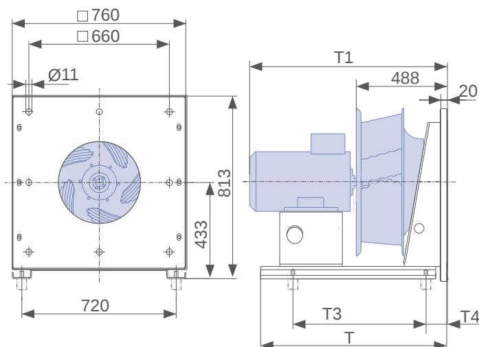
Dimensions mm
