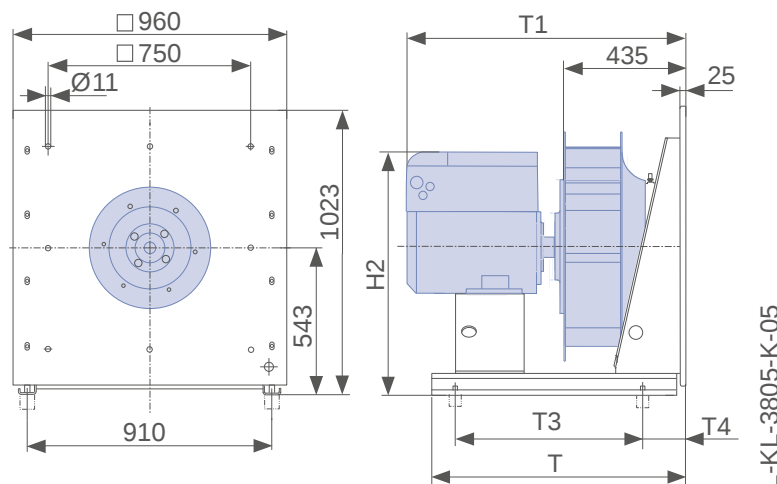
Dimensions mm
