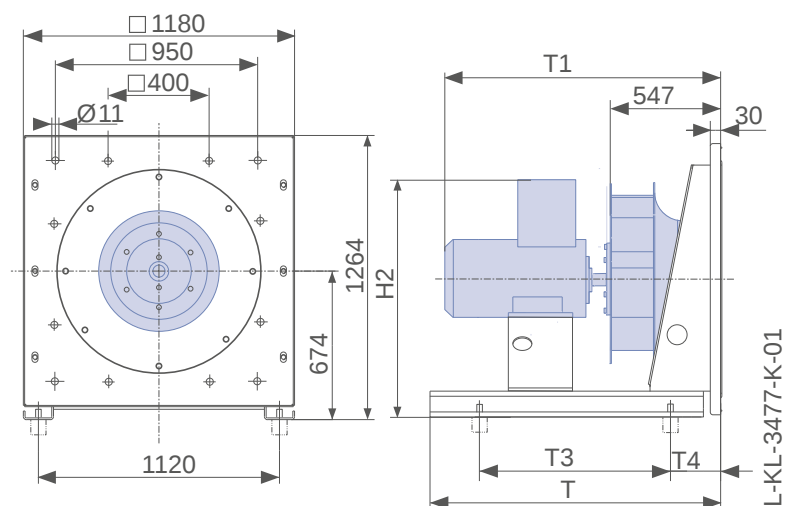
Dimensions mm
