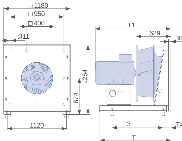
Dimensions mm
