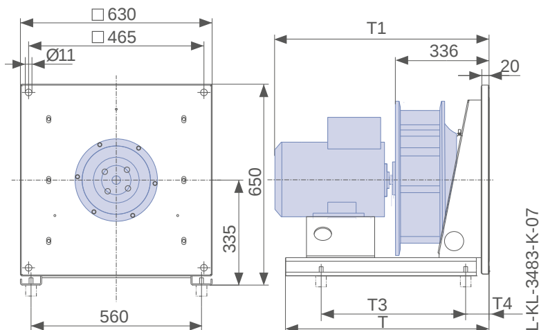
Dimensions mm
