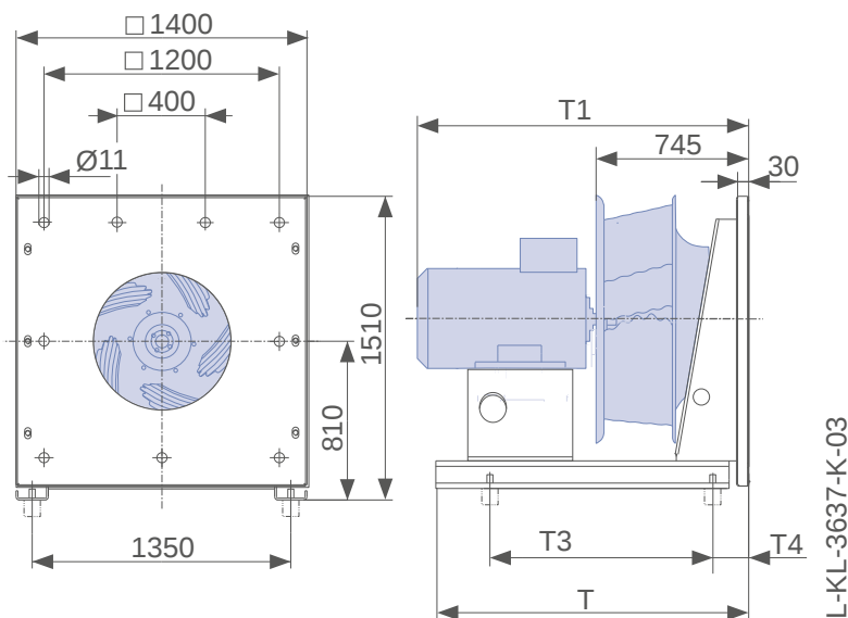
Dimensions mm
