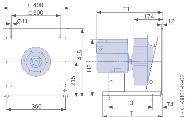
Dimensions mm
