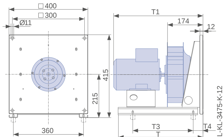
Dimensions mm
