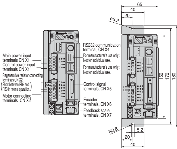
Rack mount type (Option : Front-end mounting)
