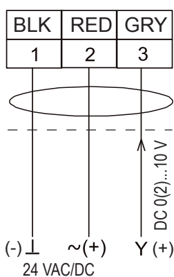
24 Vac/Vdc Proportional Model
