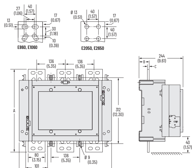
Figure 91 - 100-E860, 100-E1060, 100-E2050, 100-E2650 Contactors with PLC Input
