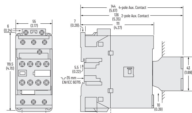
Figure 58 - 100(S)-E40...100(S)-E65 3-Pole Contactors with Front-mounted Auxiliary Contact
