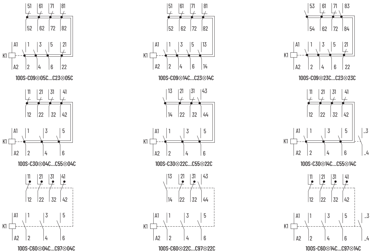
Figure 6 - Safety Contactors with 4 Main Contacts and Standard Front-mount Auxiliary Contacts
