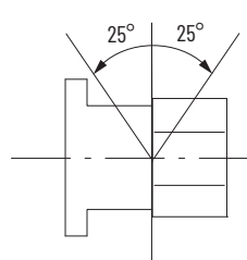
Figure 25 - Mounting Position – 100S-C DC Contactors with Conventional Coils
