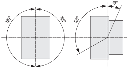
Figure 76 - 100(S)-E116K..., 100(S)-E146K... Contactors
