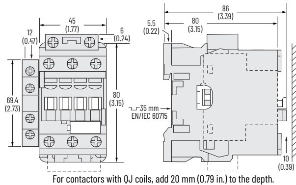
Figure 53 - 100-E26...100-E38 3-Pole Contactors with Low-consumption Coils and Side-mounted Auxiliary Contact
