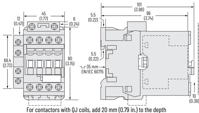
Figure 50 - 100-E26...100-E38 4-Pole Contactors with Standard Coils and Side-mounted Auxiliary Contact
