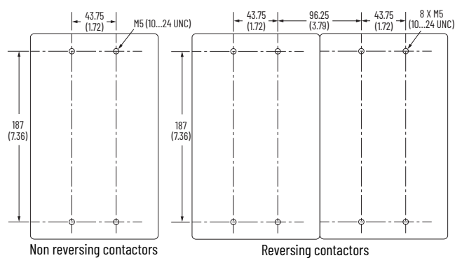
Figure 87 - Drilling Template for 265...370 A 3-Pole Contactors
