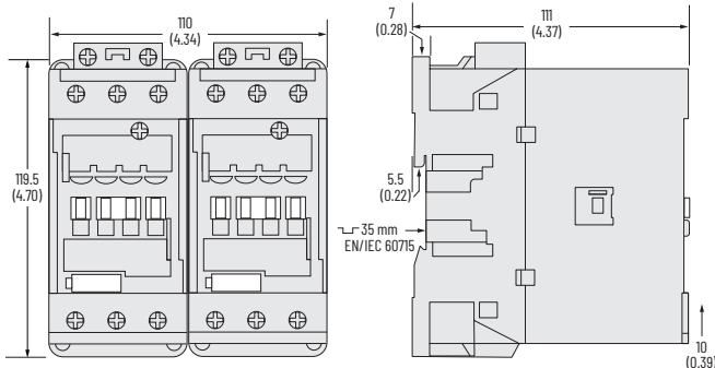
Figure 60 - 104-E40...104-E65 Reversing 3-Pole Contactors
