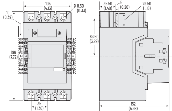
Figure 81 - 100(S)-E190E, 100(S)-E205E Contactors with PLC Input
