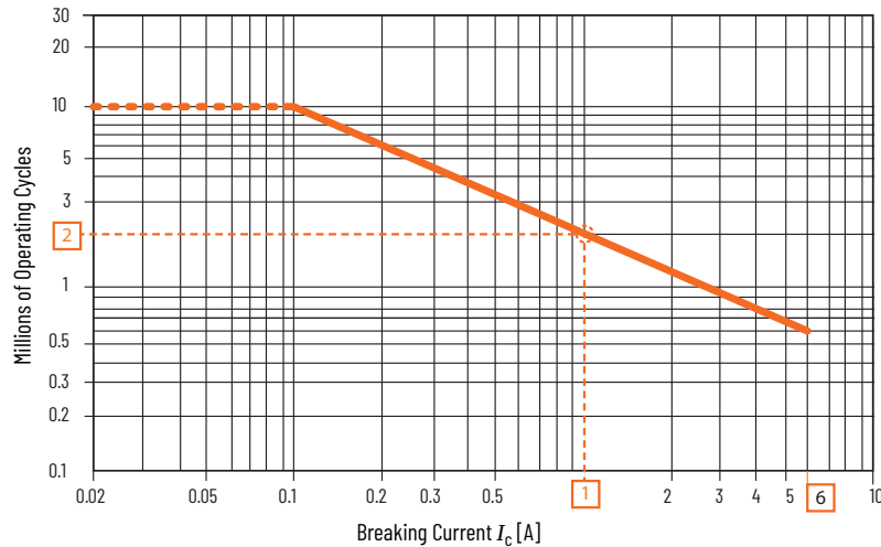
Figure 32 - Electrical Durability for DC-13 Utilization Category - U_e \leq 250V
