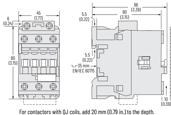
Figure 46 - 100-E26...100-E38 4-Pole Contactors with Low-consumption Coils
