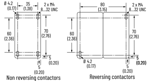
Figure 42 - Drilling Template for 9...16 A Contactors
