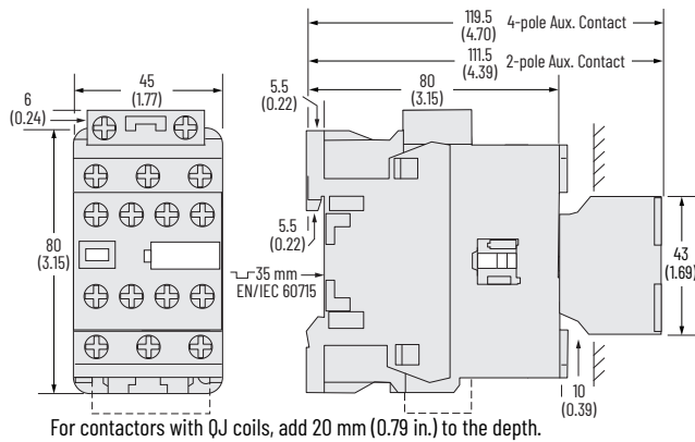
Figure 48 - 100(S)-E26...100(S)-E38 4-Pole Contactors with Standard Coils and Front-mounted Auxiliary Contact
