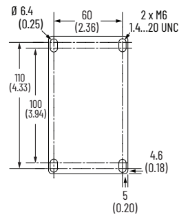
Figure 65 - Drilling Template for 40...52 A 4-Pole Contactors
