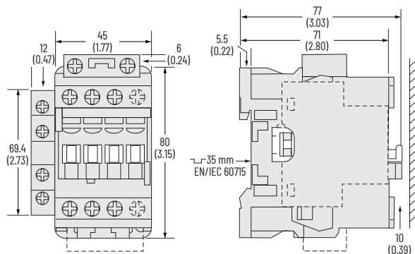
Figure 38 - 100-E09...100-E16 Contactors with Standard Coils and Side-mounted Auxiliary Contact
