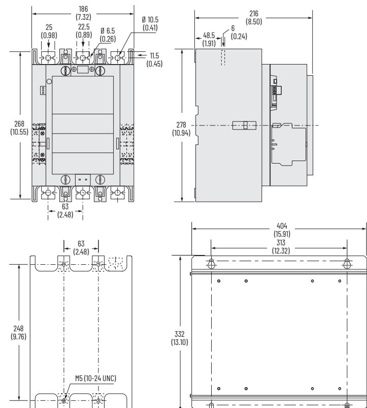
Figure 88 - 100(S)-E400, 100(S)-E460 Contactors with PLC Input
