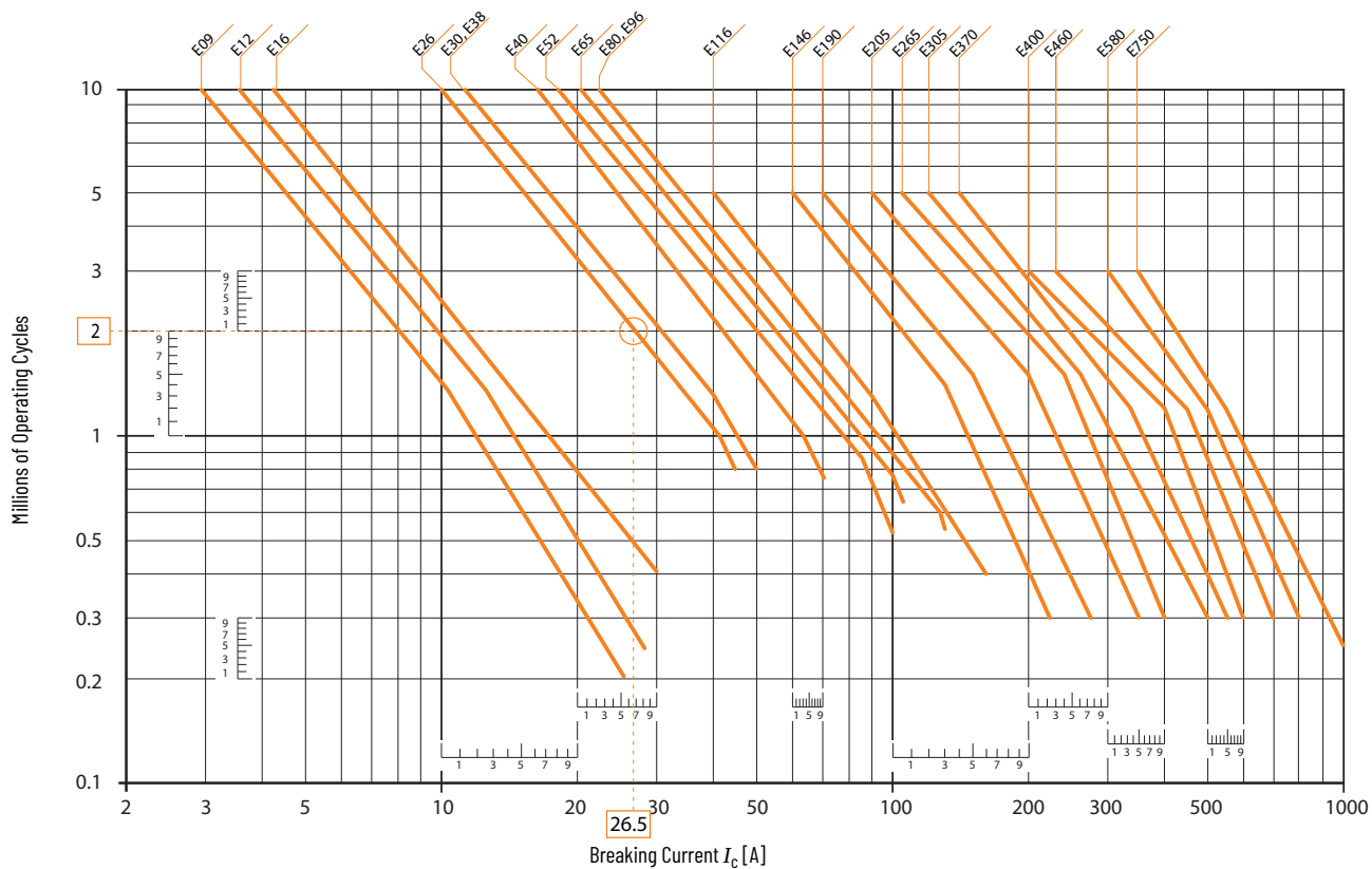
Figure 26 - Electrical Durability for AC-1 Utilization Category - U_e \leq 690V
