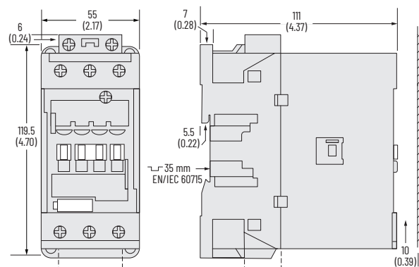
Figure 58 - 100(S)-E40...100(S)-E65 3-Pole Contactors with Front-mounted Auxiliary Contact
