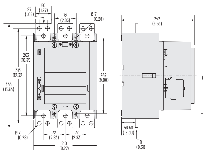
Figure 90 - 100-E1260 Contactors with PLC Input
