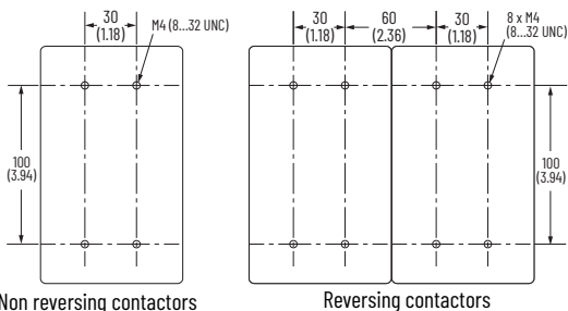
Figure 79 - Drilling Template for 116...146 A 3-Pole Contactors
