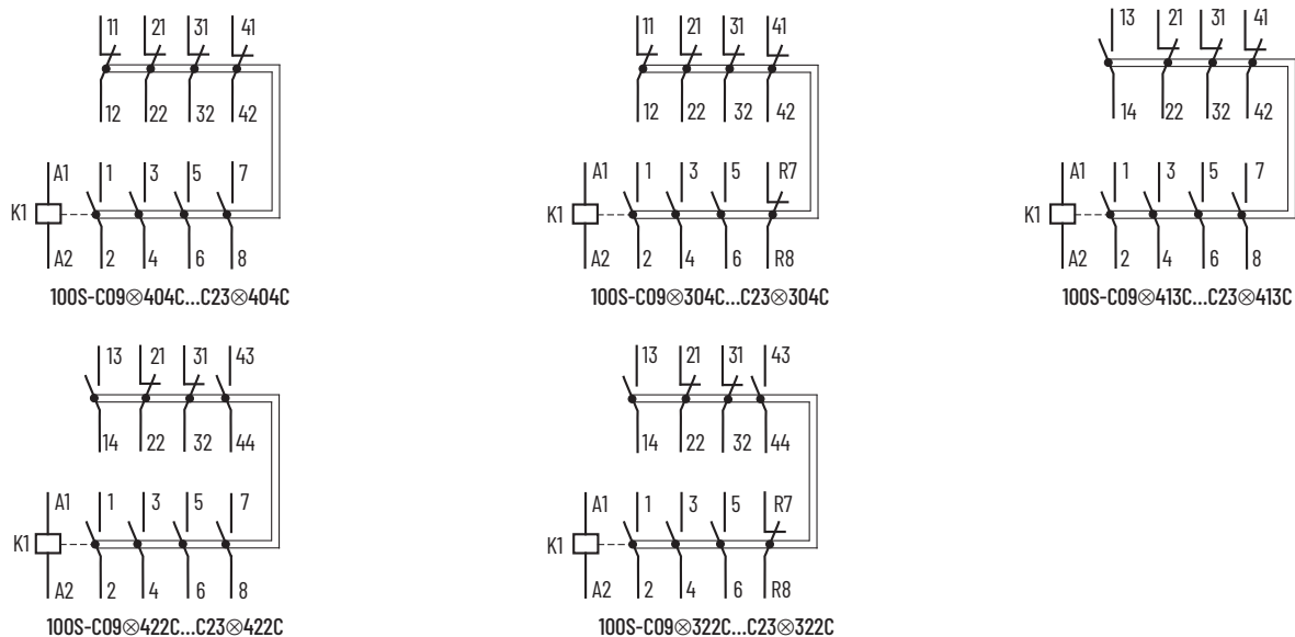
Figure 6 - Safety Contactors with 4 Main Contacts and Standard Front-mount Auxiliary Contacts
