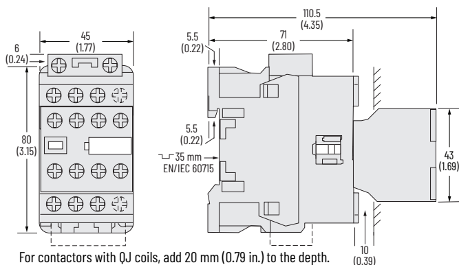
Figure 37 - 100(S)-E09...100(S)-E16 Contactors with Standard Coils and Front-mounted Auxiliary Contact
