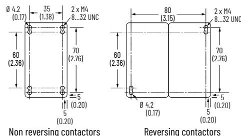
Figure 56 - Drilling Template for 26...38 A Contactors
