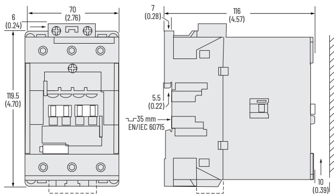
Figure 66 - 100-E80...100-E96 3-Pole Contactors
