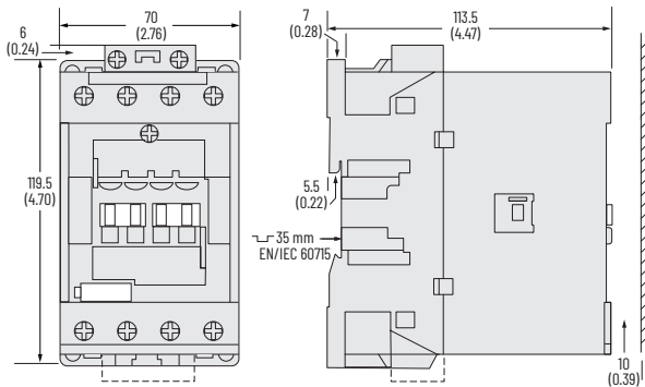
Figure 63 - 100(S)-E40...100(S)-E52 4-Pole Contactors with Front-mounted Auxiliary Contact
