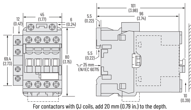
Figure 54 - 100-E26...100-E38 4-Pole Contactors with Low-consumption Coils and Side-mounted Auxiliary Contact
