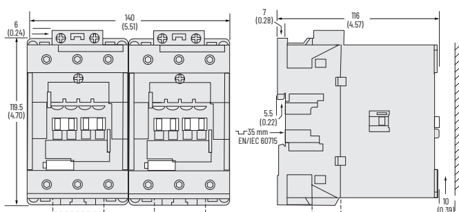
Figure 69 - 104-E80...104-E96 Reversing 3-Pole Contactors
