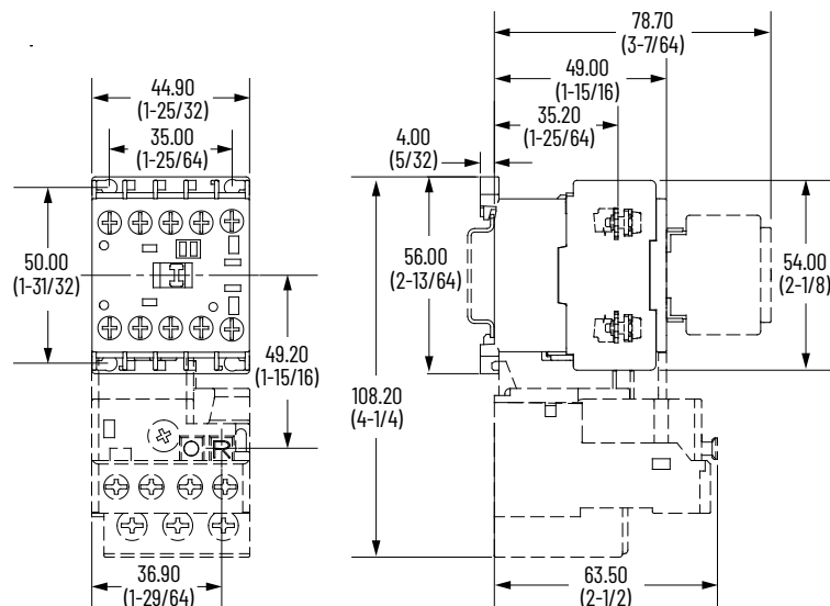
Figure 4 - Mounting Position
