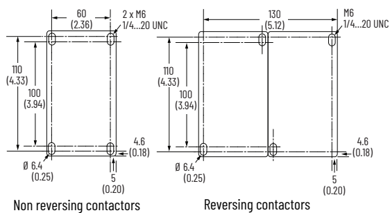
Figure 71 - 100-E80 4-Pole Contactors
