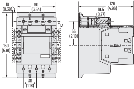
Figure 77 - 100(S)-E116E..., 100(S)-E146E... Contactors with PLC Input
