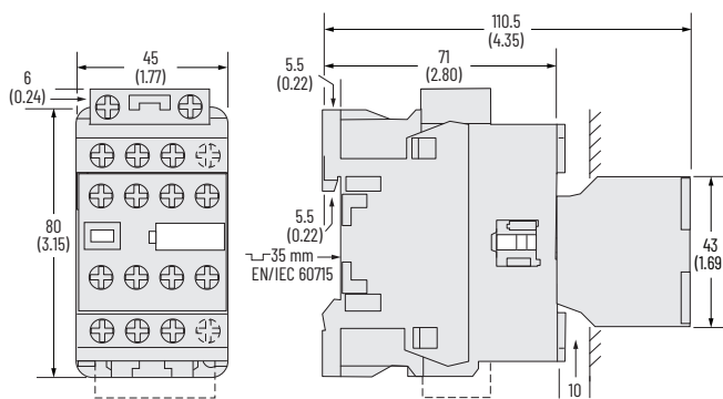
Figure 39 - 100(S)-E09...100(S)-E16 Contactors with Low-consumption Coils and Front-mounted Auxiliary Contact
