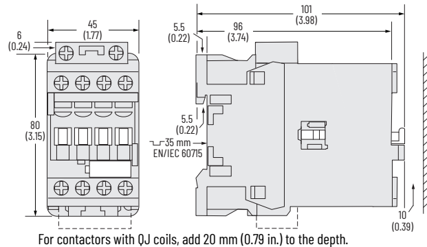
Figure 46 - 100-E26...100-E38 4-Pole Contactors with Low-consumption Coils
