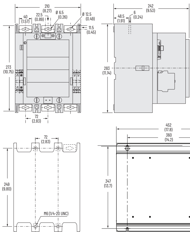
Figure 89 - 100(S)-E580...100(S)-E750 Contactors with PLC Input
