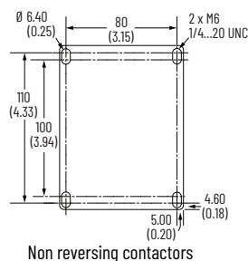
Figure 74 - Drilling Template for 80 A 4-Pole Contactors
