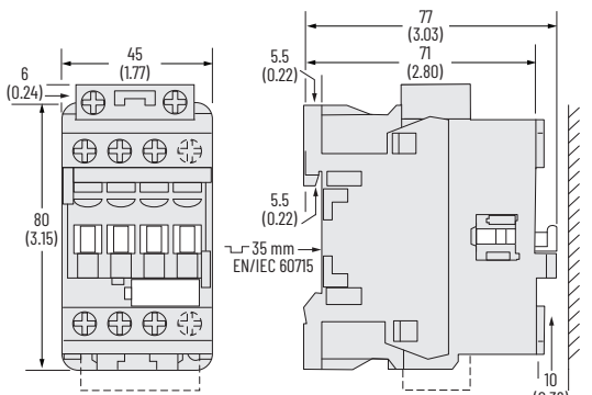
Figure 36 - 100-E09...100-E16 Contactors with Low-consumption Coils
