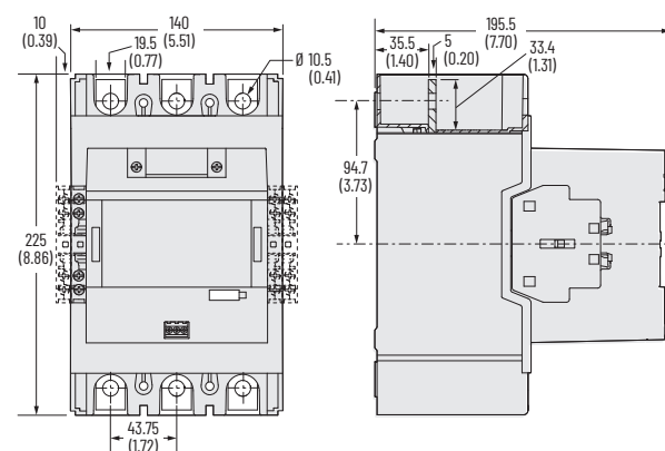
Figure 88 - 100(S)-E400, 100(S)-E460 Contactors with PLC Input
