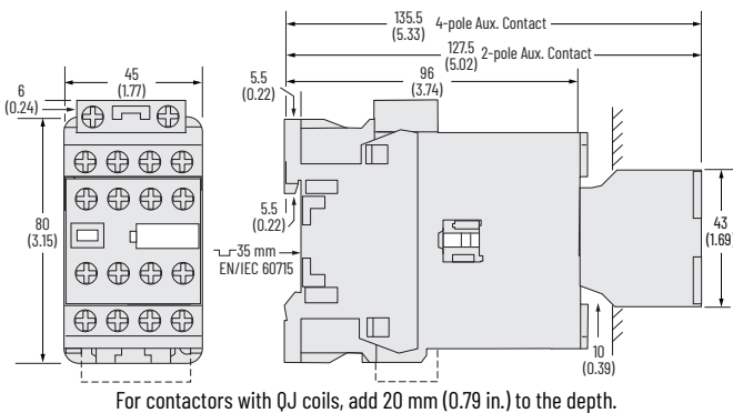
Figure 49 - 100-E26...100-E38 3-Pole Contactors with Standard Coils and Side-mounted Auxiliary Contact
