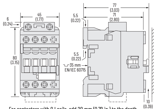
Figure 36 - 100-E09...100-E16 Contactors with Low-consumption Coils
